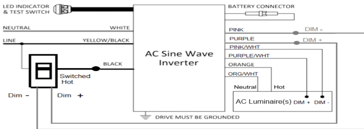
Figure A. Wiring Diagram with 0-10V Dimmer 500W Max. Connected Load
